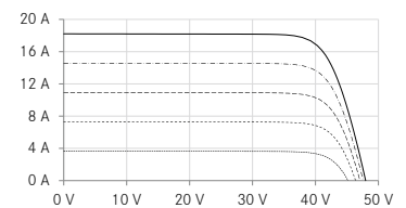
UI-diagram e.g. 680 Wp
