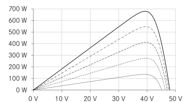
UP - diagram e.g. 680 Wp
